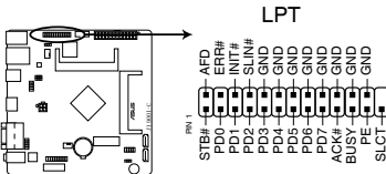
J19001-C Parallel port connector
