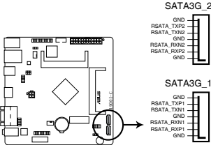
J1900I-C SATA 3.0Gb/s connectors
