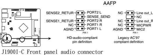
J19001-C Front panel audio connector
