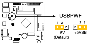
J1900I-C USB device wake up
