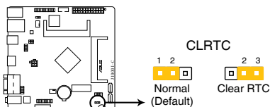
J1900I-C Clear RTC RAM
