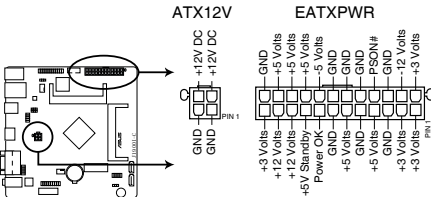
J19001-C ATX power connectors
