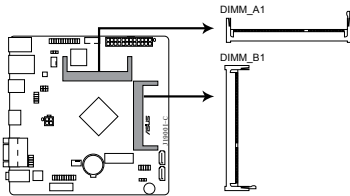
J1900I-C 204-pin DDR3 SO-DIMM sockets
