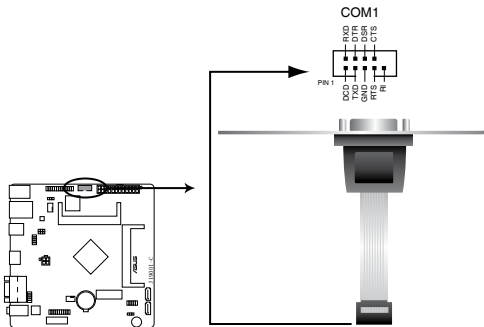
J19001-C Serial port connectors
