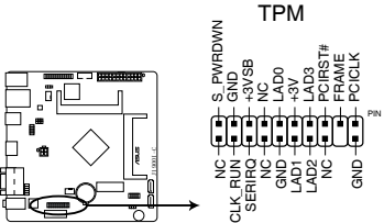
J1900I-C TPM connector
