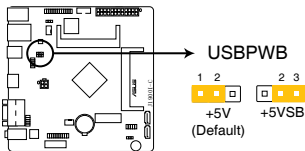
J1900I-C USB device wake up
