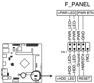
J19001-C System panel connector
