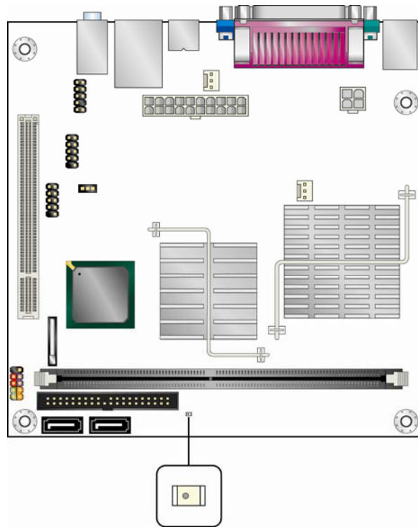
Figure 5. Location of the Standby Power Indicator LED
