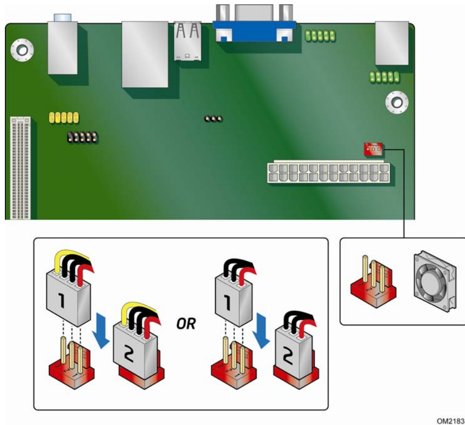
Figure 11. Location of the Chassis Fan Header
