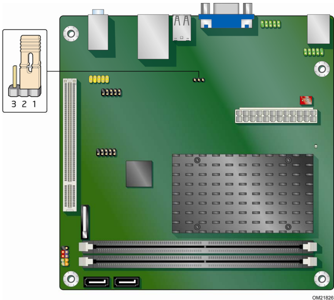
Figure 13. BIOS Configuration Jumper Block
