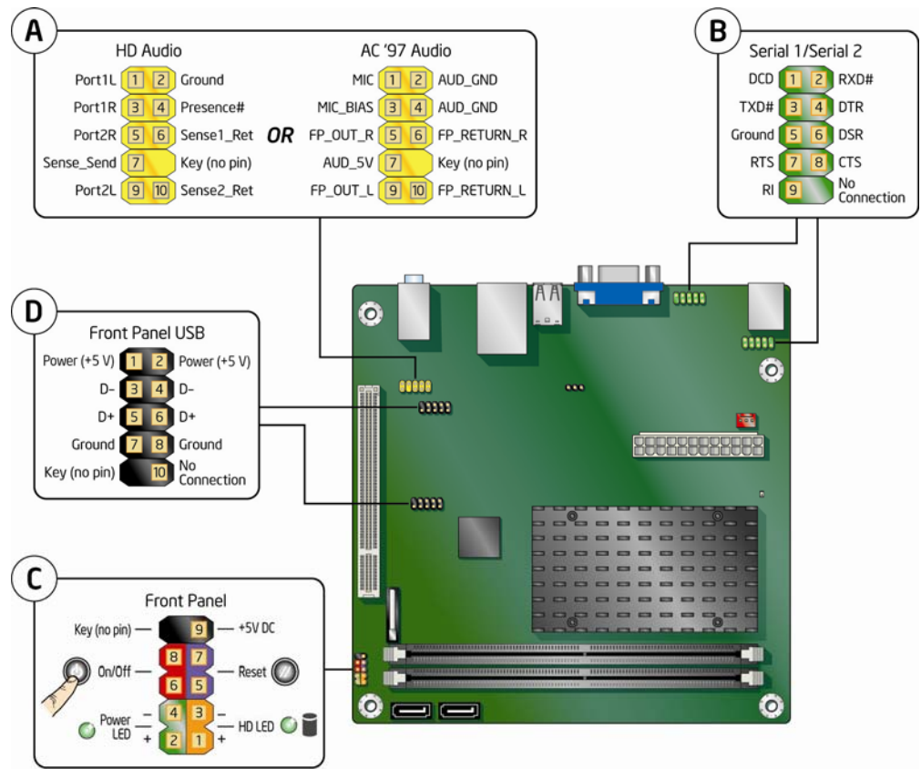
Figure 10. Internal Headers
