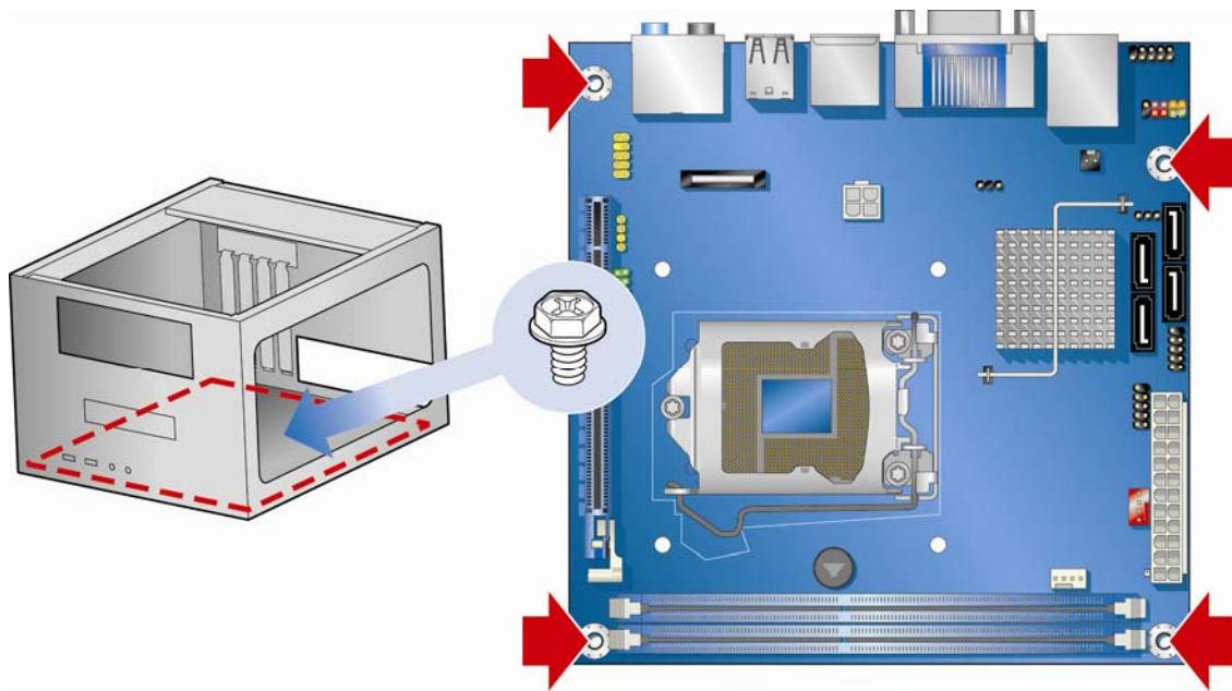
Figure 5. Intel Desktop Board DH57JG Mounting Screw Hole Locations
