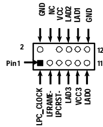
LPC1 Connector
