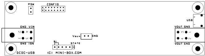
Fig 1.0, DCDC-USB layout
