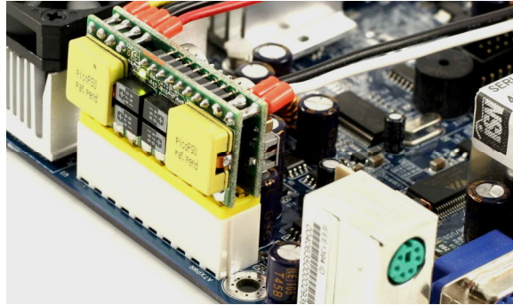
Fig 1.1 picoPSU-120 plugged into ATX connector.
